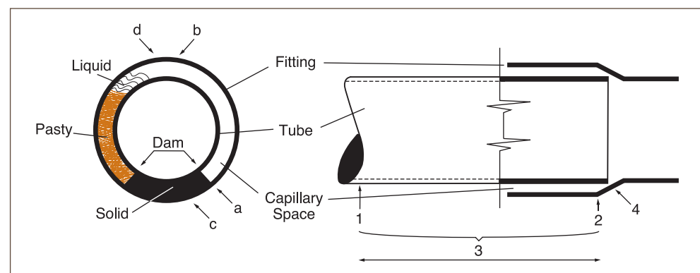
Figure 7.18. Schematic of Solder Joint
