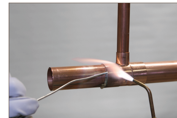
Figure 7.16. Soldering
