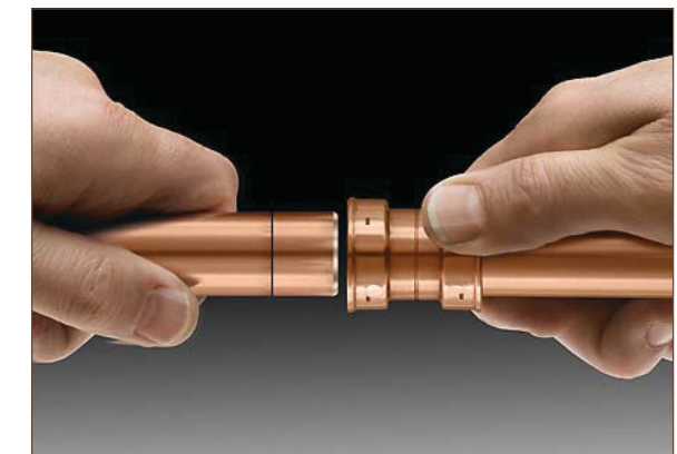
Figure 12.11. Aligning tube end squarely
