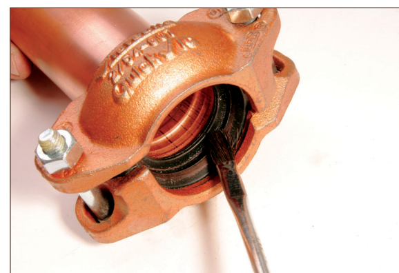
Figure 10.8. Applying lubrication to gasket
