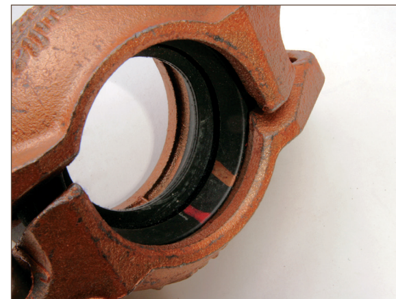
Figure 10.6. Clamp and gasket assembly
