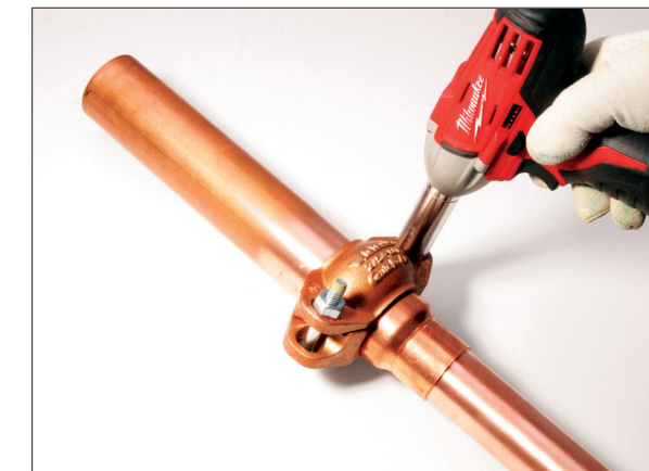
Figure 10.11. Tightening the clamp
