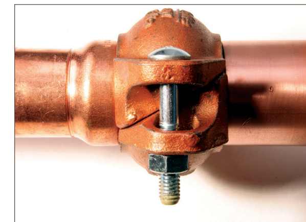
Figure 10.12. Final inspection of completed joint
