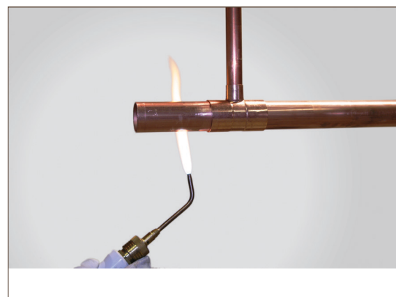
Figure 7.13. Preheating Tube
