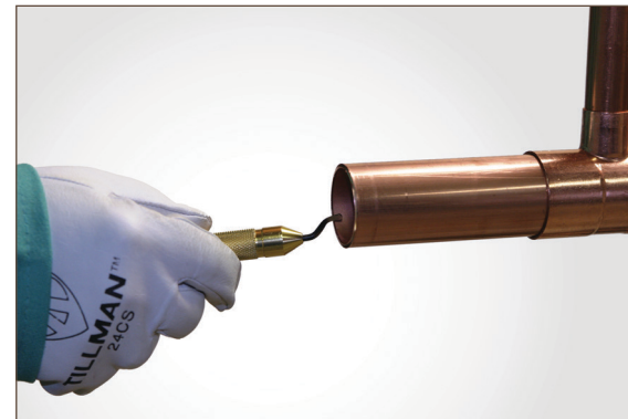
Figure 7.5. Reaming: Deburring Tool
