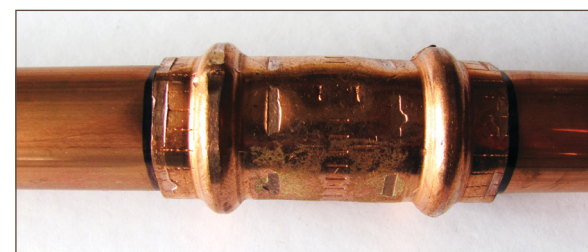
Figure 11.16. Completed installation of a press-connect joint
