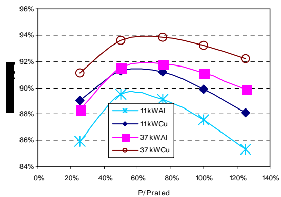
Fig. 2 – Efficiency vs. Load, 11 and 37 kW.
