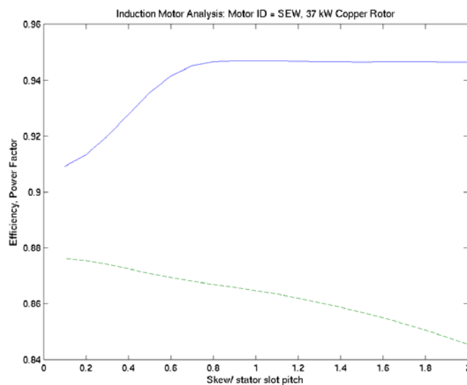
Fig. 6 – Effect of rotor skew on motor efficiency (solid) and power factor (dashed) for the 37-kW copper rotor motor.
