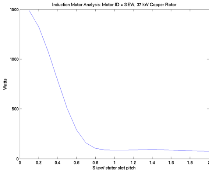
Fig. 5 – Effect of rotor skew on stray load losses for the 37-kW copper rotor motor.
