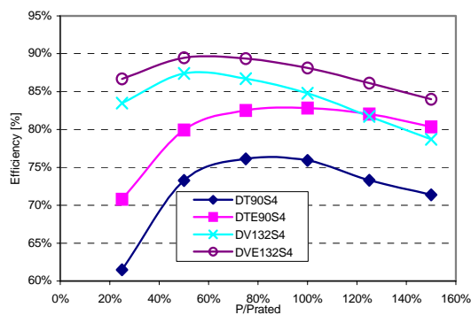
Fig. 1 - Efficiency vs. Load, 1.1 and 5.5 kW.
