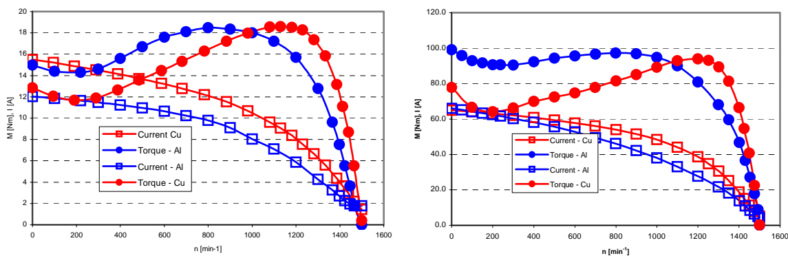
Fig. 3 – Torque-speed and current-speed curves for the 1.1 kW motors (left) and 5.5 kW motors (right). Standard efficiency aluminium motor (blue); high efficiency copper motor (red).
