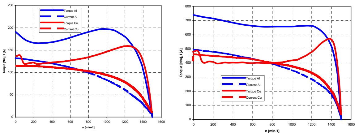
Fig. 4 – Torque-speed and current-speed curves for the 11 kW motors (left) and 37 kW motors (right). Standard efficiency aluminium motor (blue); high efficiency copper motor (red).
